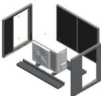
Lateral Panel
