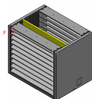
Screwing
