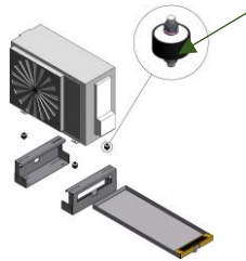
Silent Block M8 Ø40 H20 Washer Ø8x24 Nut M8
