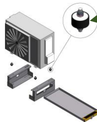
Heat pump supports + silentblocks + condensate drain pan
