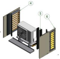
Side panels with big and small acoustic grid
