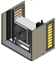
Side panels with big and small acoustic grid
